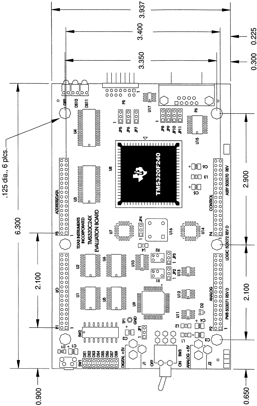
Figure A-1. TMS320C24x Evaluation Board
